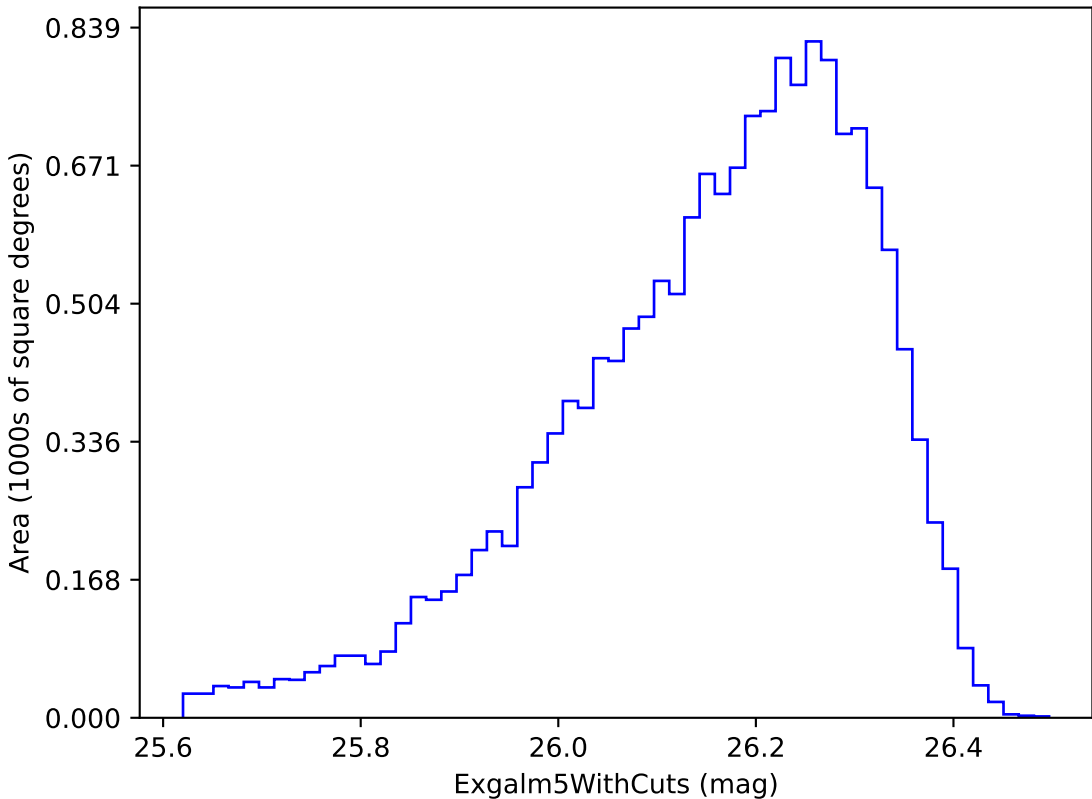
noroll_mjdp365_v3.4_10yrs i band non-DD year 6: ExgalM5WithCuts
