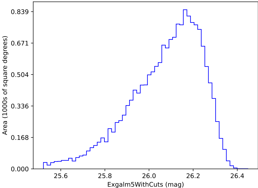
noroll_mjdp365_v3.4_10yrs i band non-DD year 5: ExgalM5WithCuts
