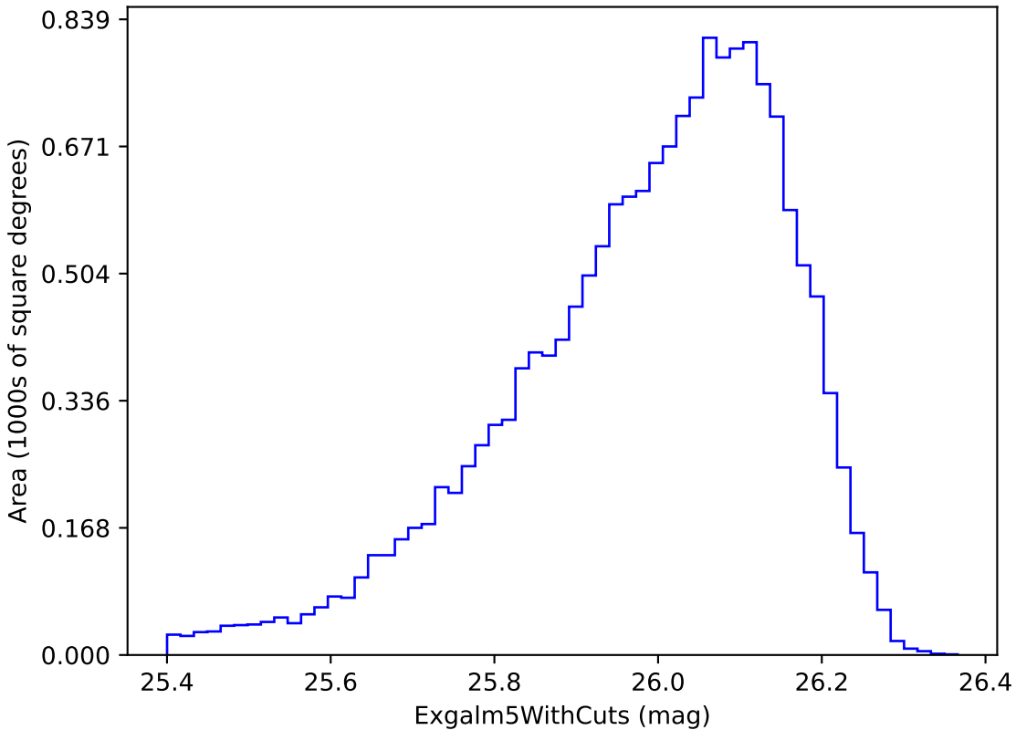
noroll_mjdp365_v3.4_10yrs i band non-DD year 4: ExgalM5WithCuts
