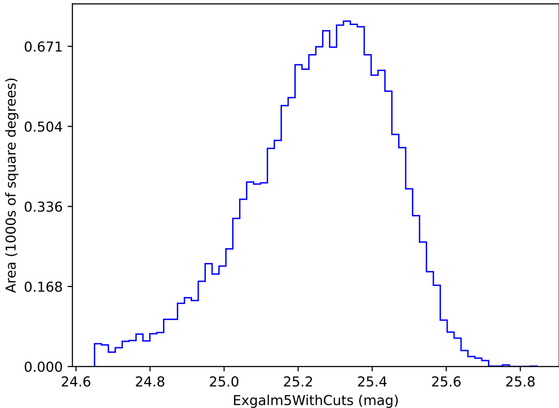
noroll_mjdp365_v3.4_10yrs i band non-DD year 1: ExgalM5WithCuts
