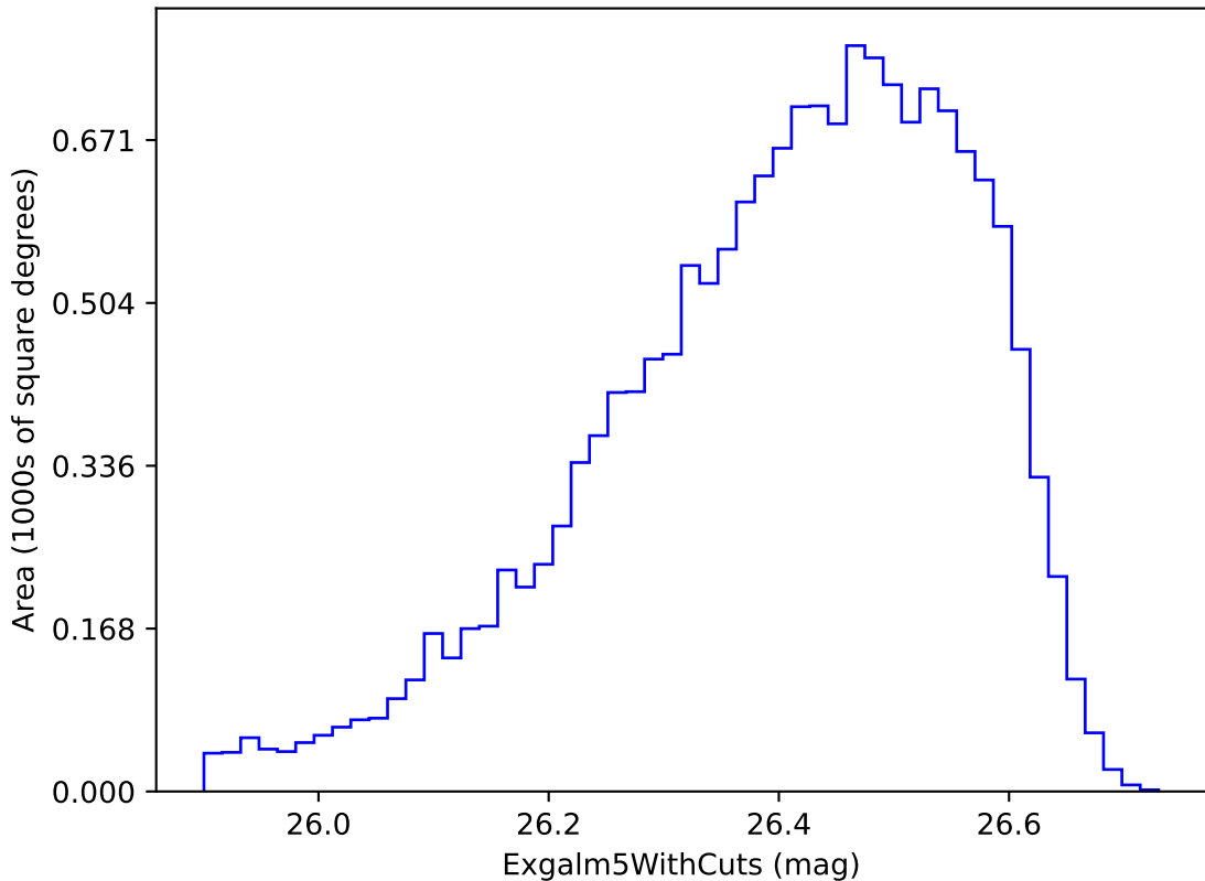
noroll_mjdp365_v3.4_10yrs i band non-DD year 10: Exgal5WithCuts
