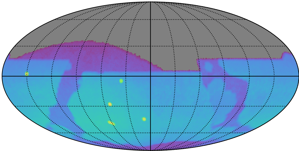
noroll_mjdp365_v3.4_10yrs : Brown Dwarf, L7
