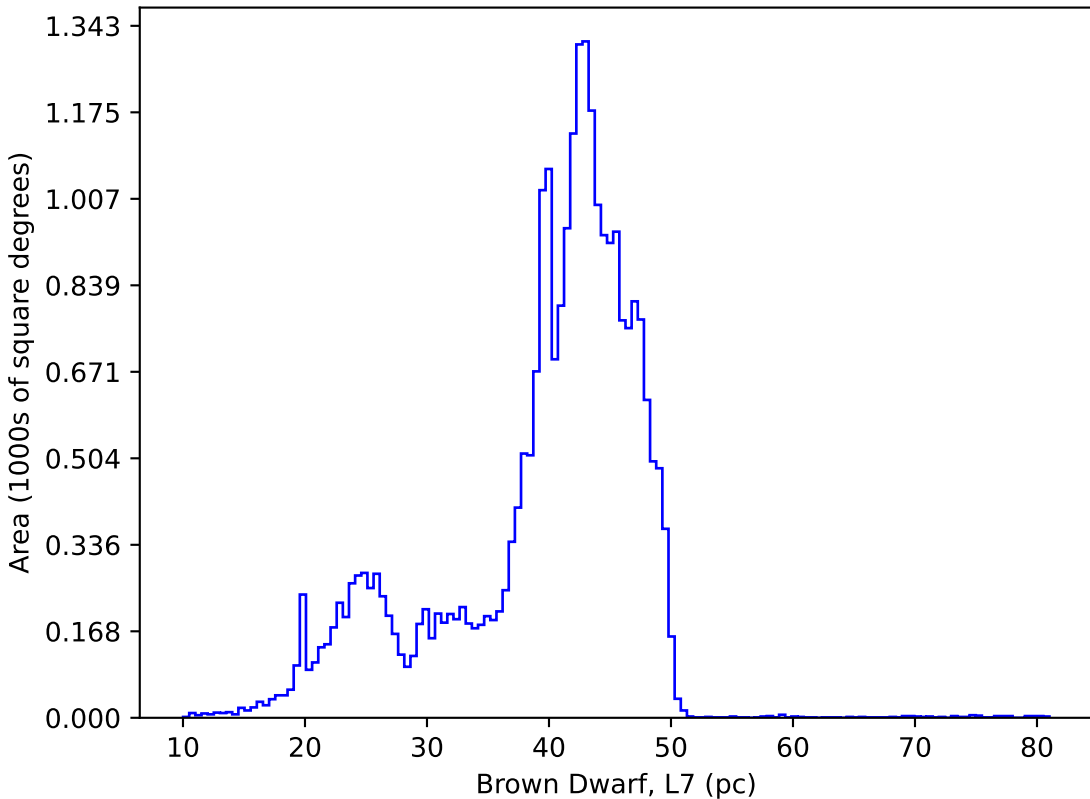
noroll_mjdp365_v3.4_10yrs : Brown Dwarf, L7
