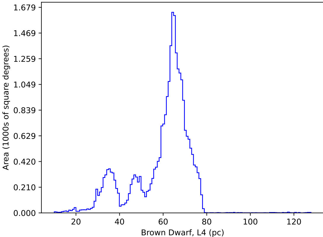
noroll_mjdp365_v3.4_10yrs : Brown Dwarf, L4
