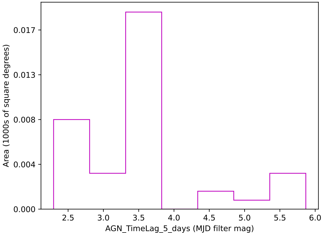
noroll_mjdp365_v3.4_10yrs z band: AGN_TimeLag_5_days
