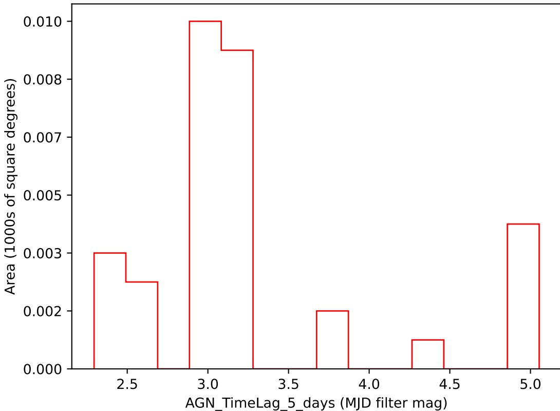
noroll_mjdp365_v3.4_10yrs i band: AGN_TimeLag_5_days
