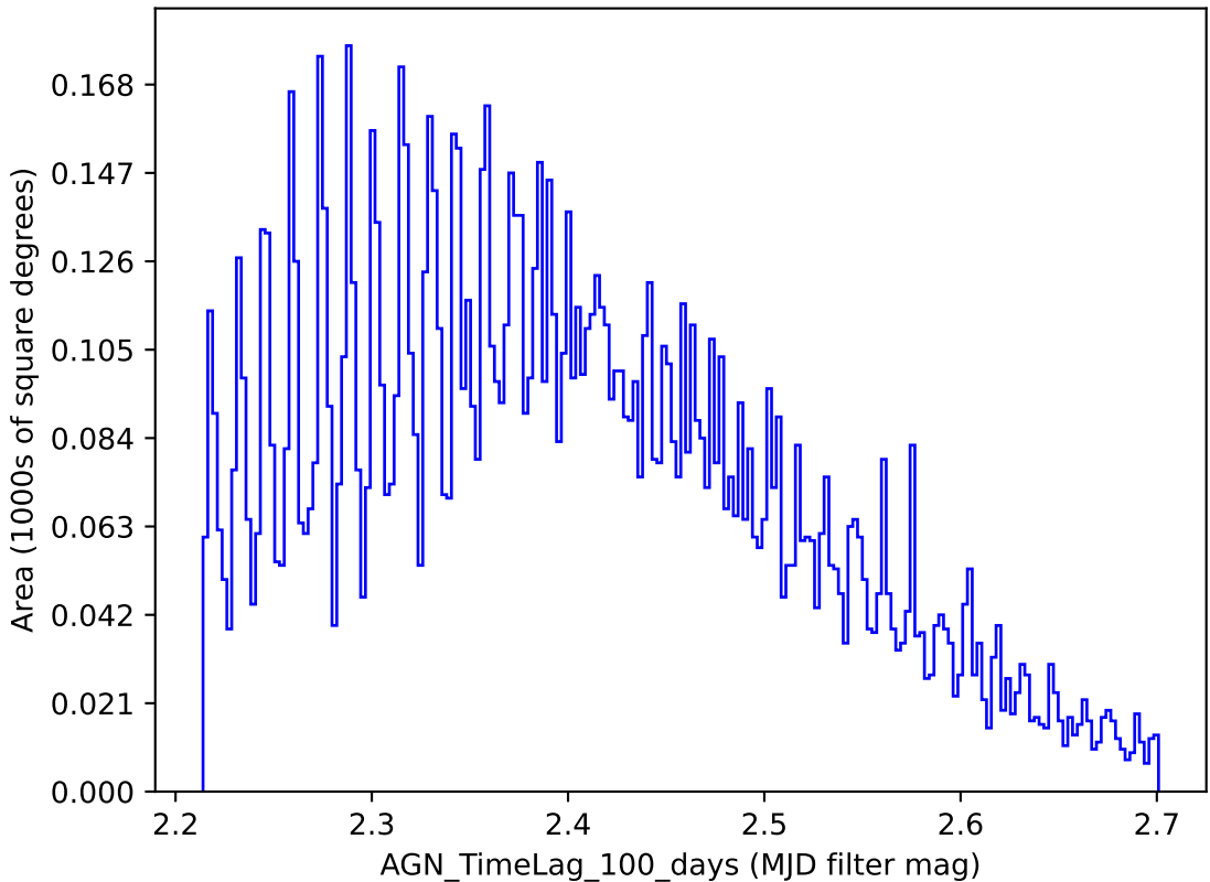
noroll_mjdp365_v3.4_10yrs y band: AGN_TimeLag_100_days
