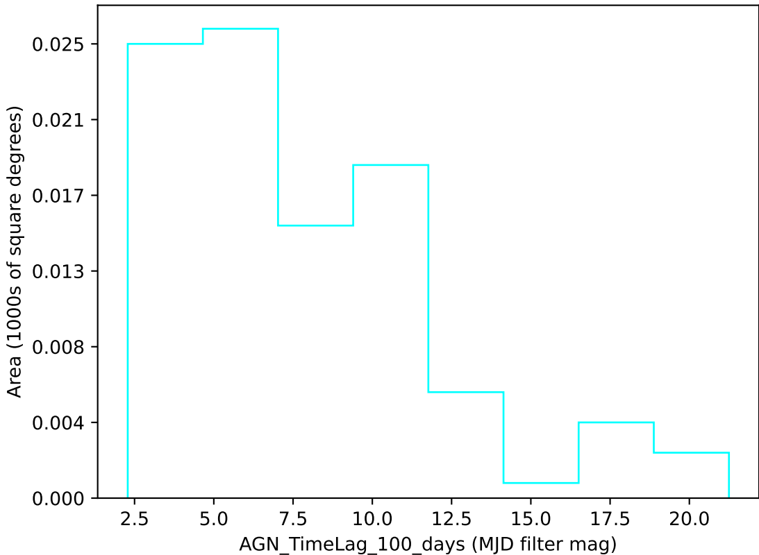
noroll_mjdp365_v3.4_10yrs u band: AGN_TimeLag_100_days
