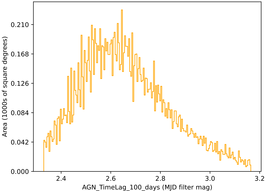
noroll_mjdp365_v3.4_10yrs r band: AGN_TimeLag_100_days
