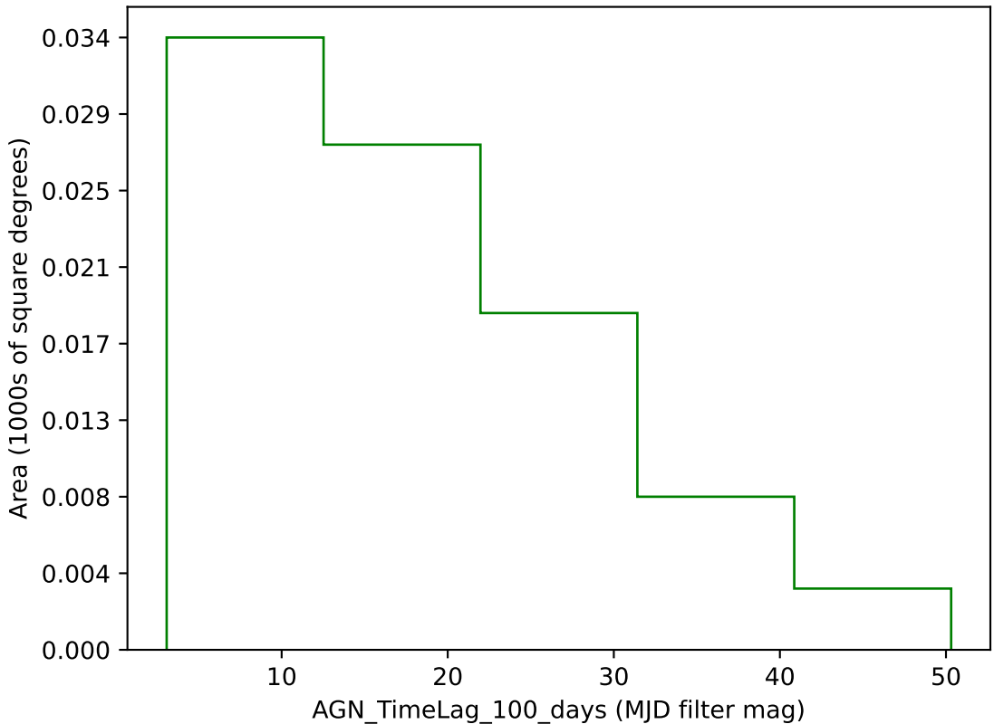
noroll_mjdp365_v3.4_10yrs g band: AGN_TimeLag_100_days
