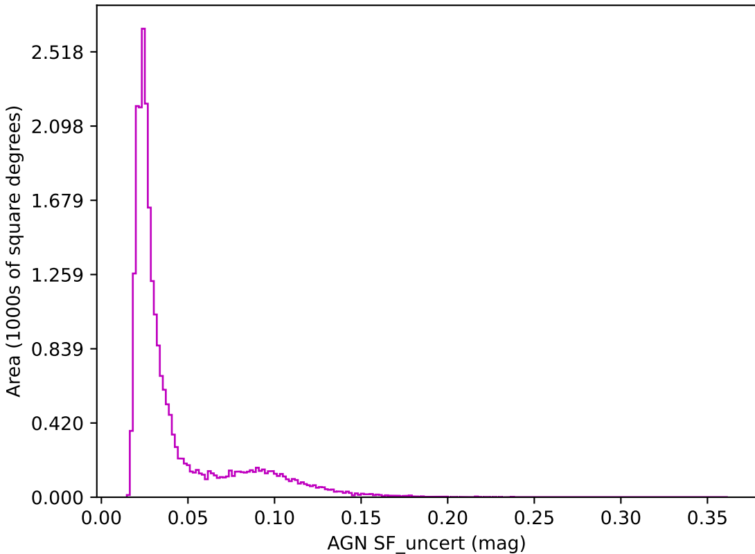
noroll_mjdp365_v3.4_10yrs z band: AGN SF_uncert
