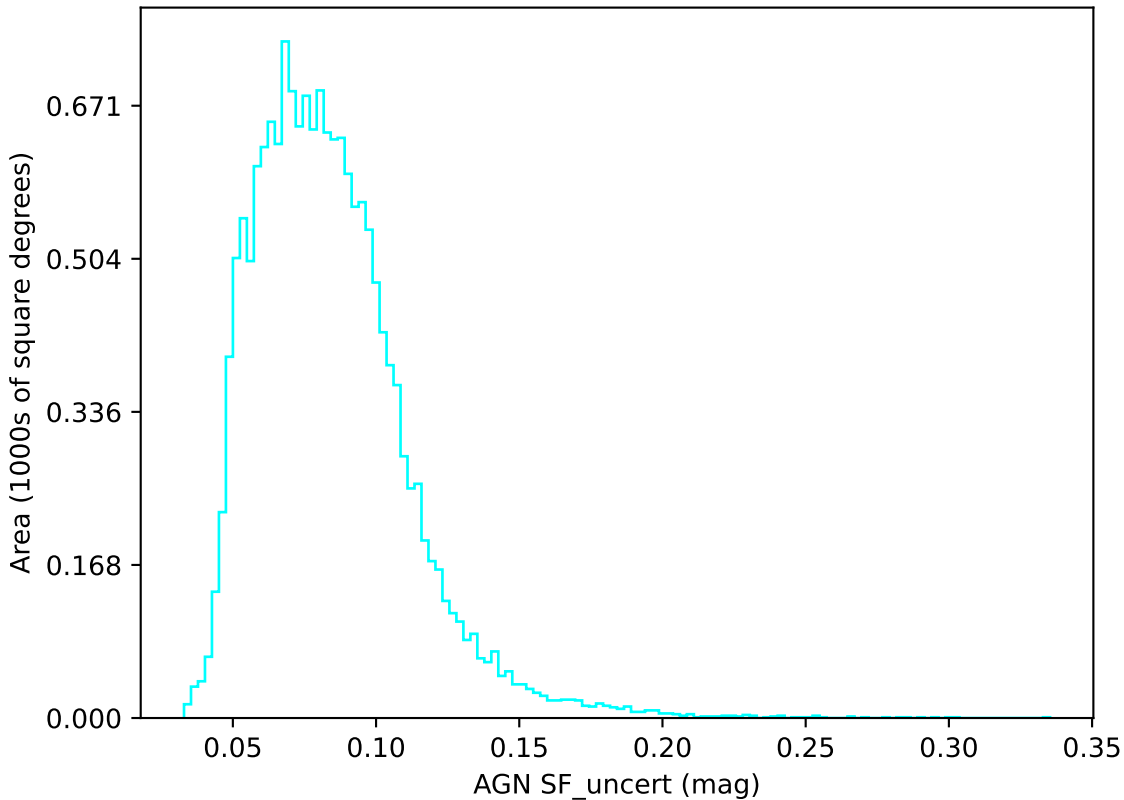
noroll_mjdp365_v3.4_10yrs u band: AGN SF_uncert
