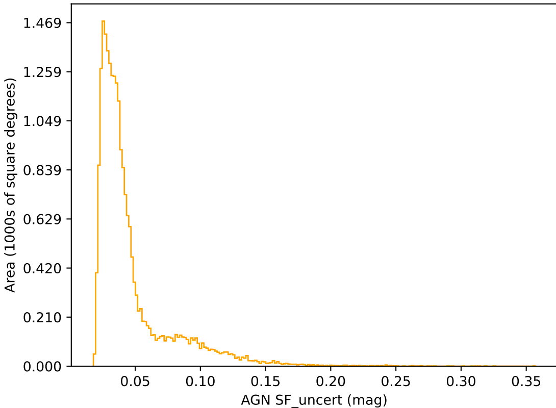
noroll_mjdp365_v3.4_10yrs r band: AGN SF_uncert
