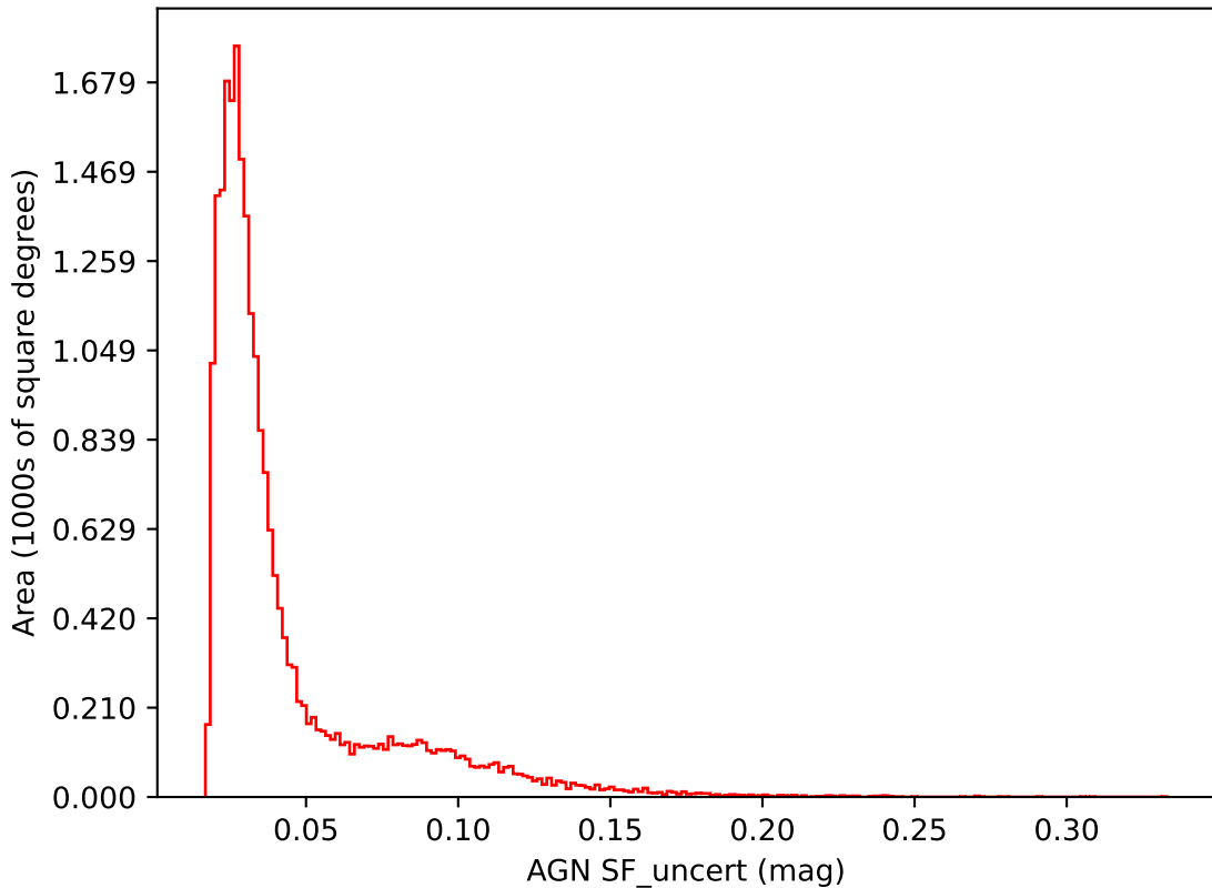
noroll_mjdp365_v3.4_10yrs i band: AGN SF_uncert
