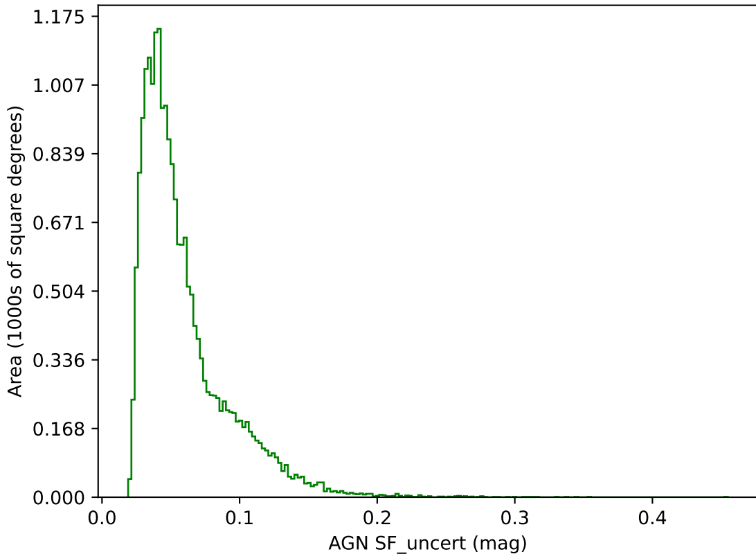
noroll_mjdp365_v3.4_10yrs g band: AGN SF_uncert
