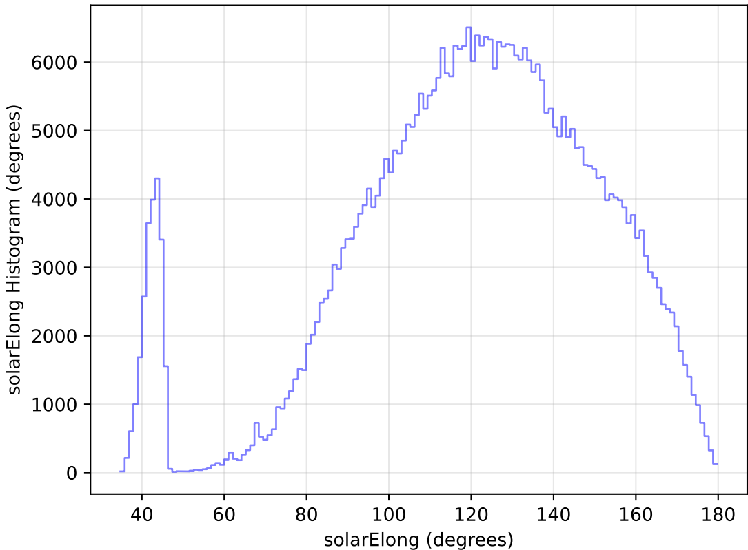
noroll_mjdp365_v3.4_10yrs WFD z band: solarElong Histogram
