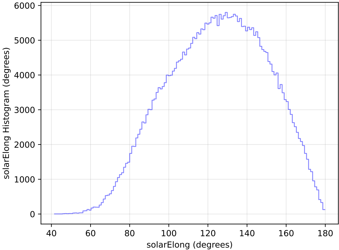
noroll_mjdp365_v3.4_10yrs WFD y band: solarElong Histogram
