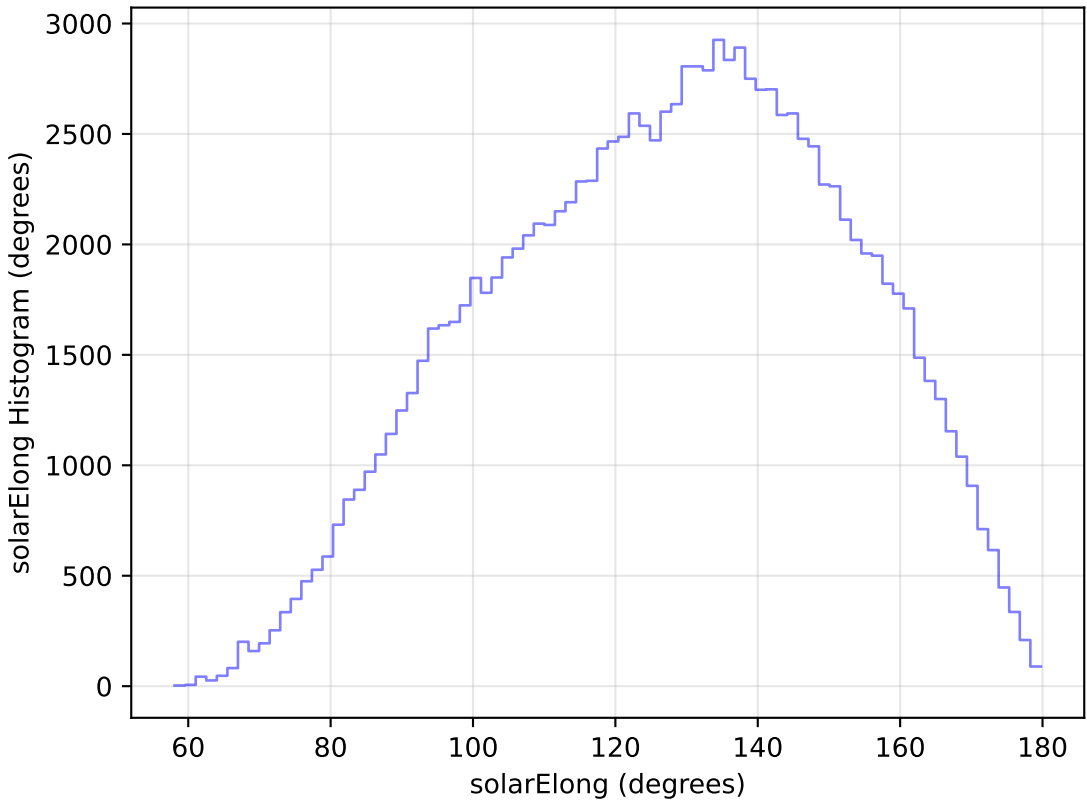
noroll_mjdp365_v3.4_10yrs WFD u band: solarElong Histogram
