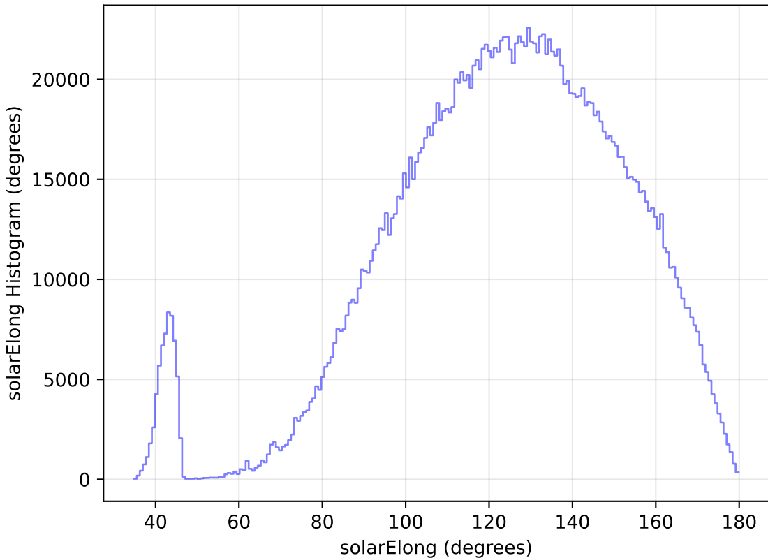
noroll_mjdp365_v3.4_10yrs WFD all bands: solarElong Histogram
