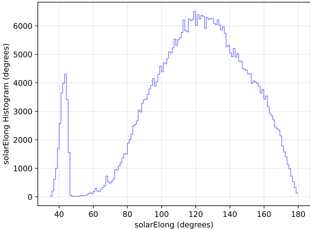
noroll_mjdp365_v3.4_10yrs All sky z band: solarElong Histogram
