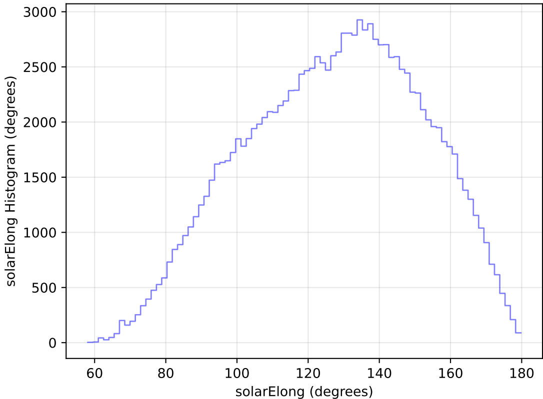
noroll_mjdp365_v3.4_10yrs All sky u band: solarElong Histogram
