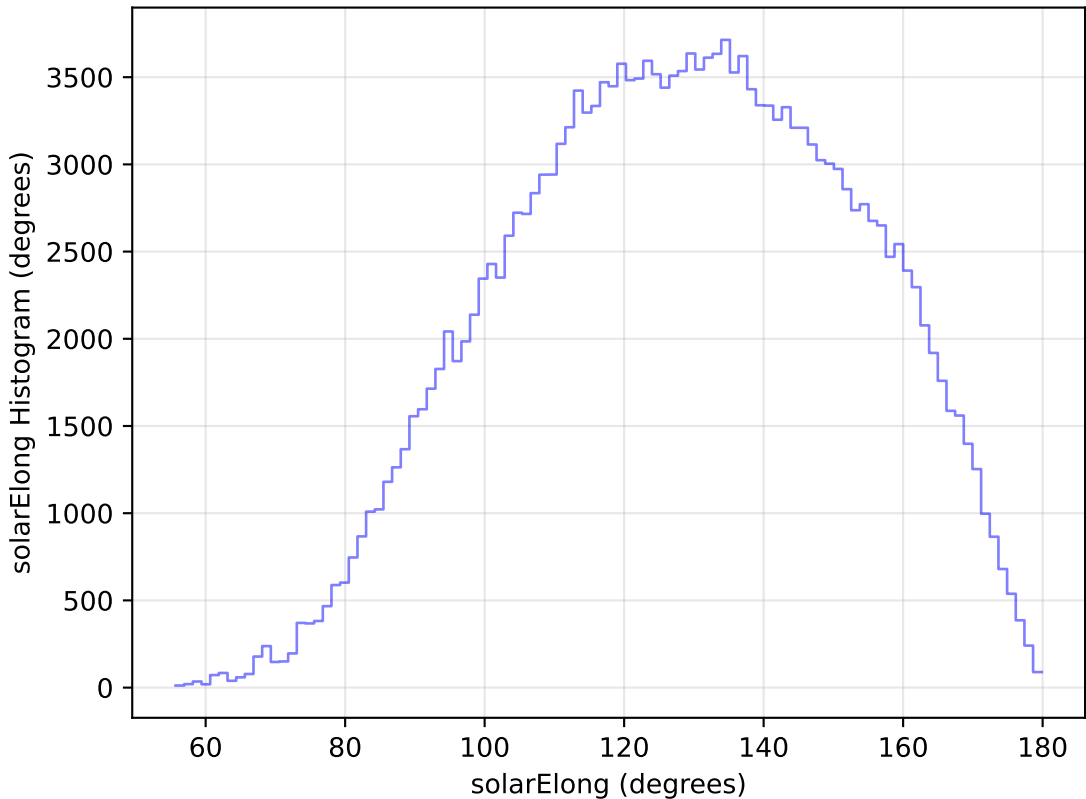
noroll_mjdp365_v3.4_10yrs All sky g band: solarElong Histogram
