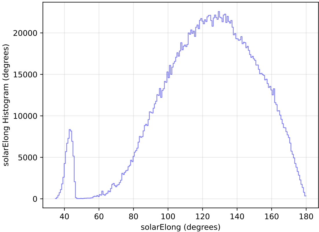
noroll_mjdp365_v3.4_10yrs All sky all bands: solarElong Histogram
