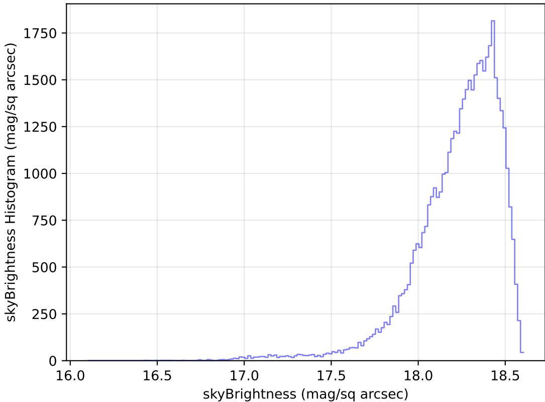
noroll_mjdp365_v3.4_10yrs Yr 1 y band: skyBrightness Histogram
