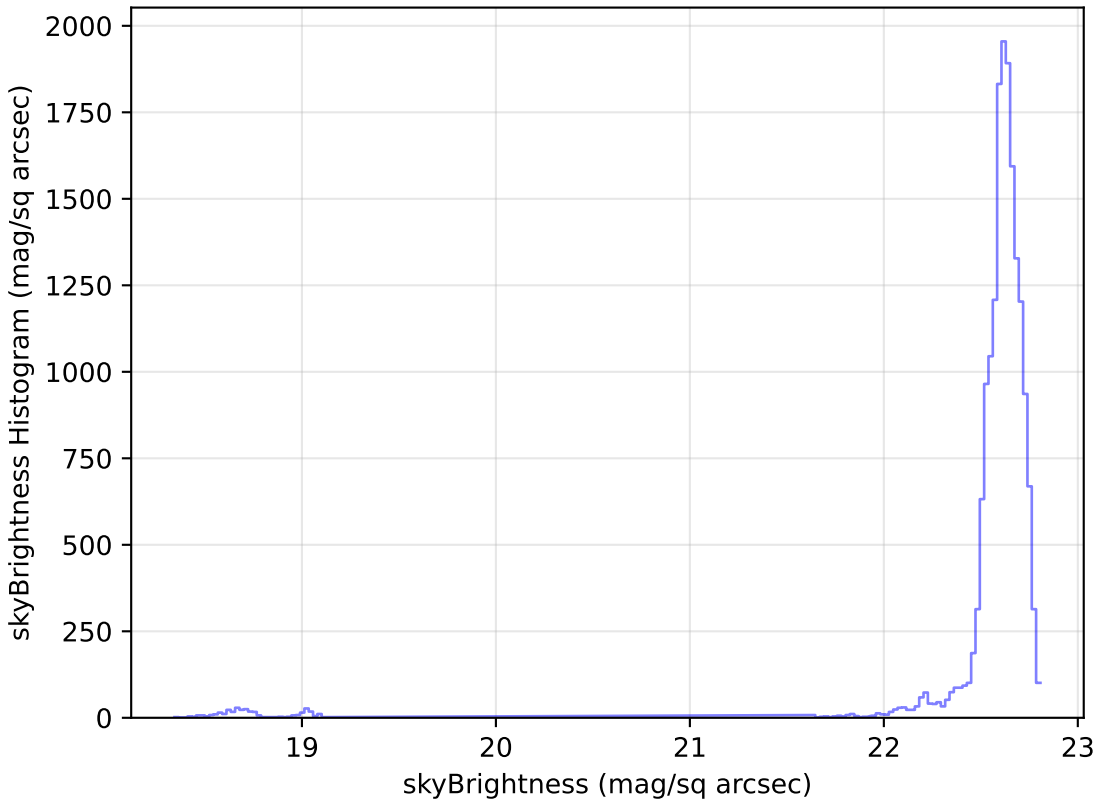
noroll_mjdp365_v3.4_10yrs Yr 1 u band: skyBrightness Histogram
