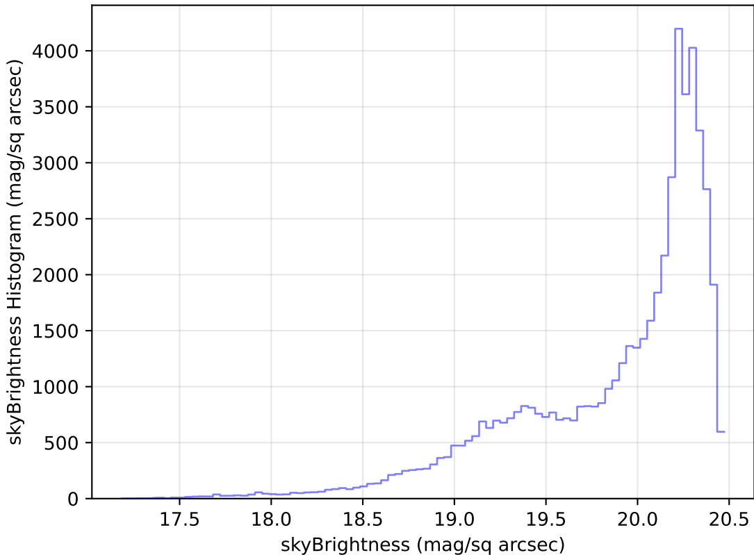
noroll_mjdp365_v3.4_10yrs Yr 1 i band: skyBrightness Histogram
