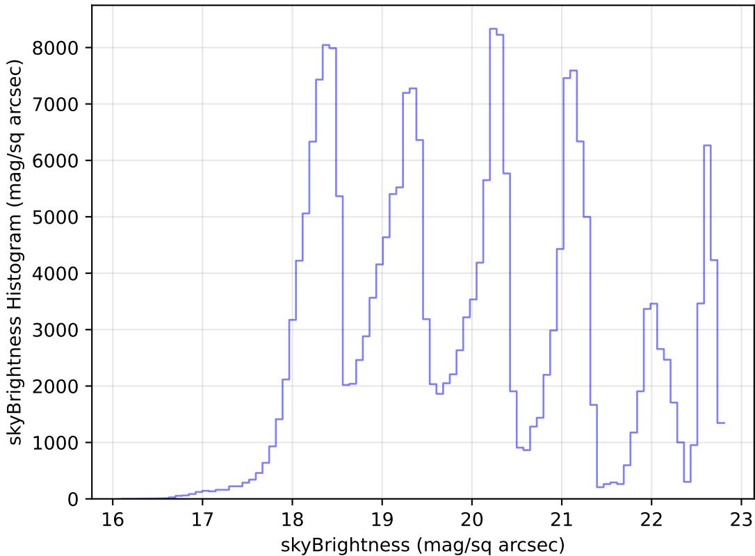
noroll_mjdp365_v3.4_10yrs Yr 1 all bands: skyBrightness Histogram
