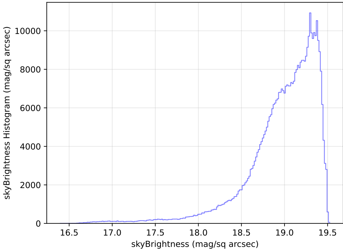
noroll_mjdp365_v3.4_10yrs WFD z band: skyBrightness Histogram
