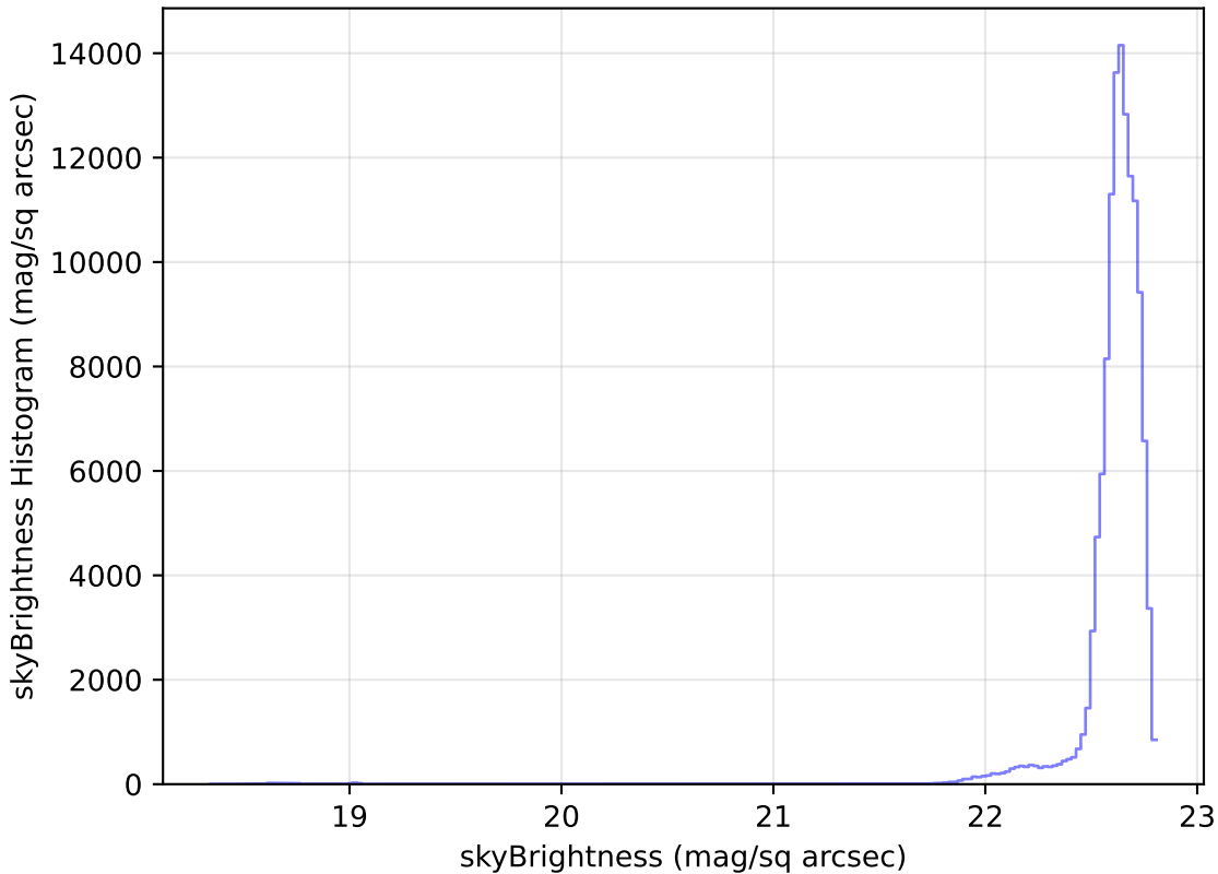
noroll_mjdp365_v3.4_10yrs WFD u band: skyBrightness Histogram
