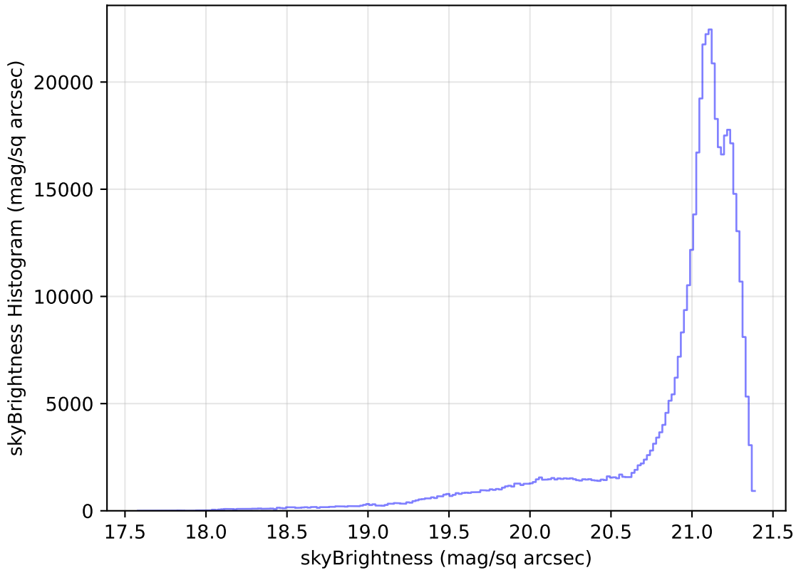
noroll_mjdp365_v3.4_10yrs WFD r band: skyBrightness Histogram
