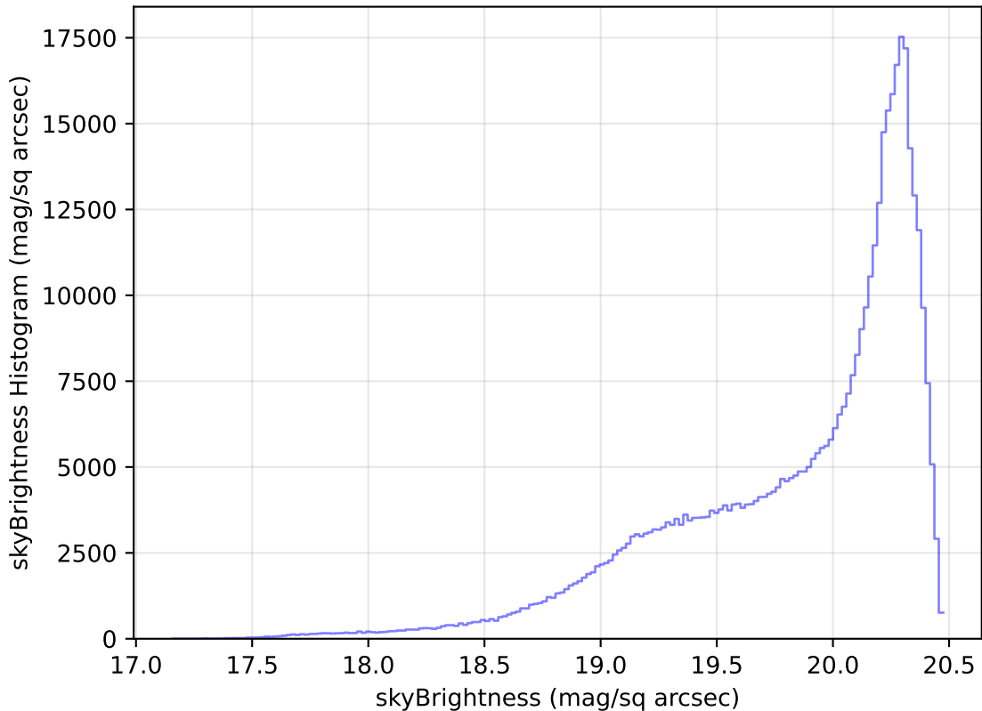
noroll_mjdp365_v3.4_10yrs WFD i band: skyBrightness Histogram
