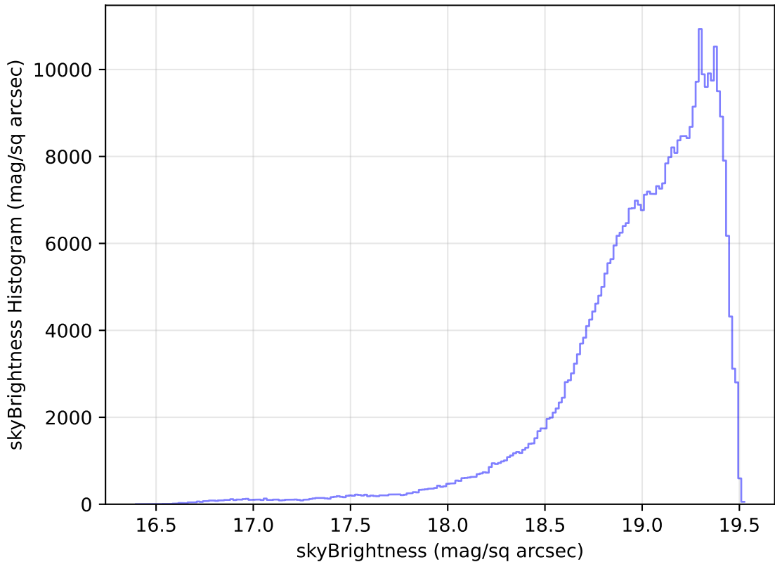
noroll_mjdp365_v3.4_10yrs All sky z band: skyBrightness Histogram
