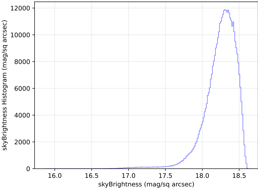
noroll_mjdp365_v3.4_10yrs All sky y band: skyBrightness Histogram
