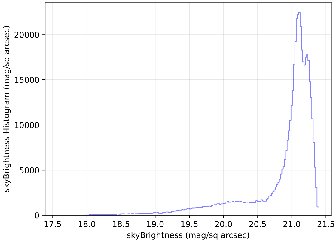
noroll_mjdp365_v3.4_10yrs All sky r band: skyBrightness Histogram
