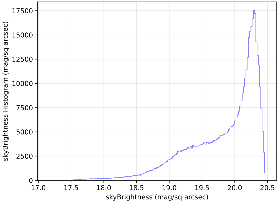
noroll_mjdp365_v3.4_10yrs All sky i band: skyBrightness Histogram
