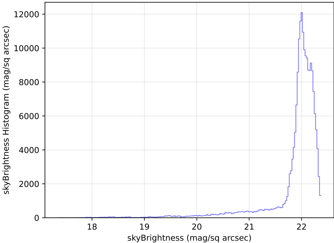
noroll_mjdp365_v3.4_10yrs All sky g band: skyBrightness Histogram
