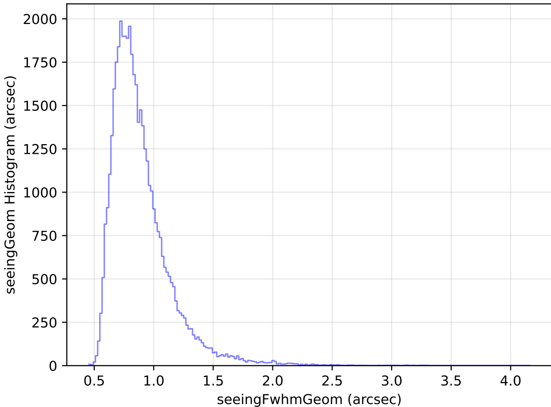
noroll_mjdp365_v3.4_10yrs Yr 1 z band: seeingGeom Histogram
