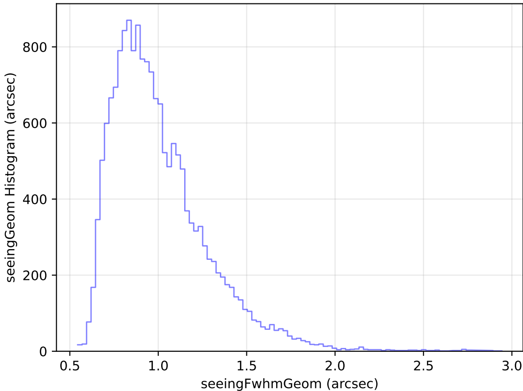
noroll_mjdp365_v3.4_10yrs Yr 1 u band: seeingGeom Histogram
