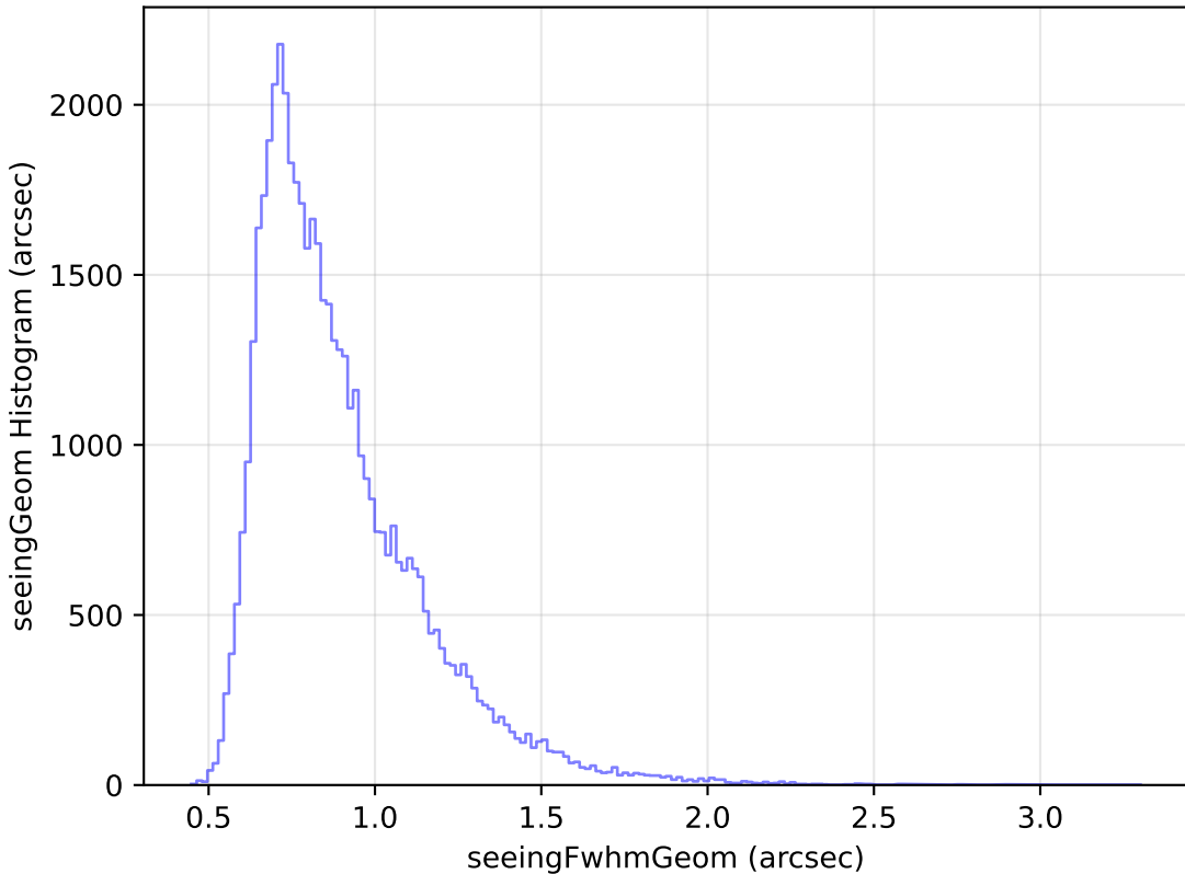
noroll_mjdp365_v3.4_10yrs Yr 1 r band: seeingGeom Histogram
