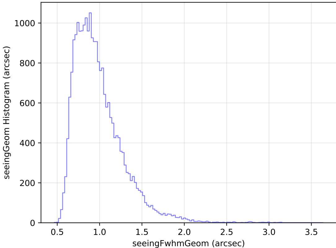
noroll_mjdp365_v3.4_10yrs Yr 1 g band: seeingGeom Histogram
