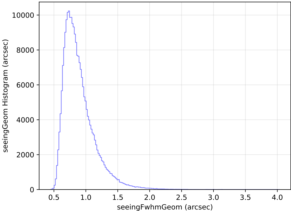
noroll_mjdp365_v3.4_10yrs Yr 1 all bands: seeingGeom Histogram
