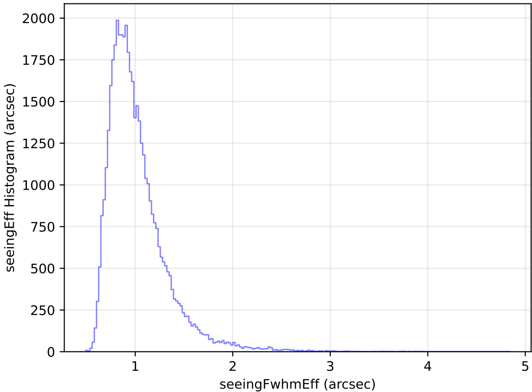
noroll_mjdp365_v3.4_10yrs Yr 1 z band: seeingEff Histogram
