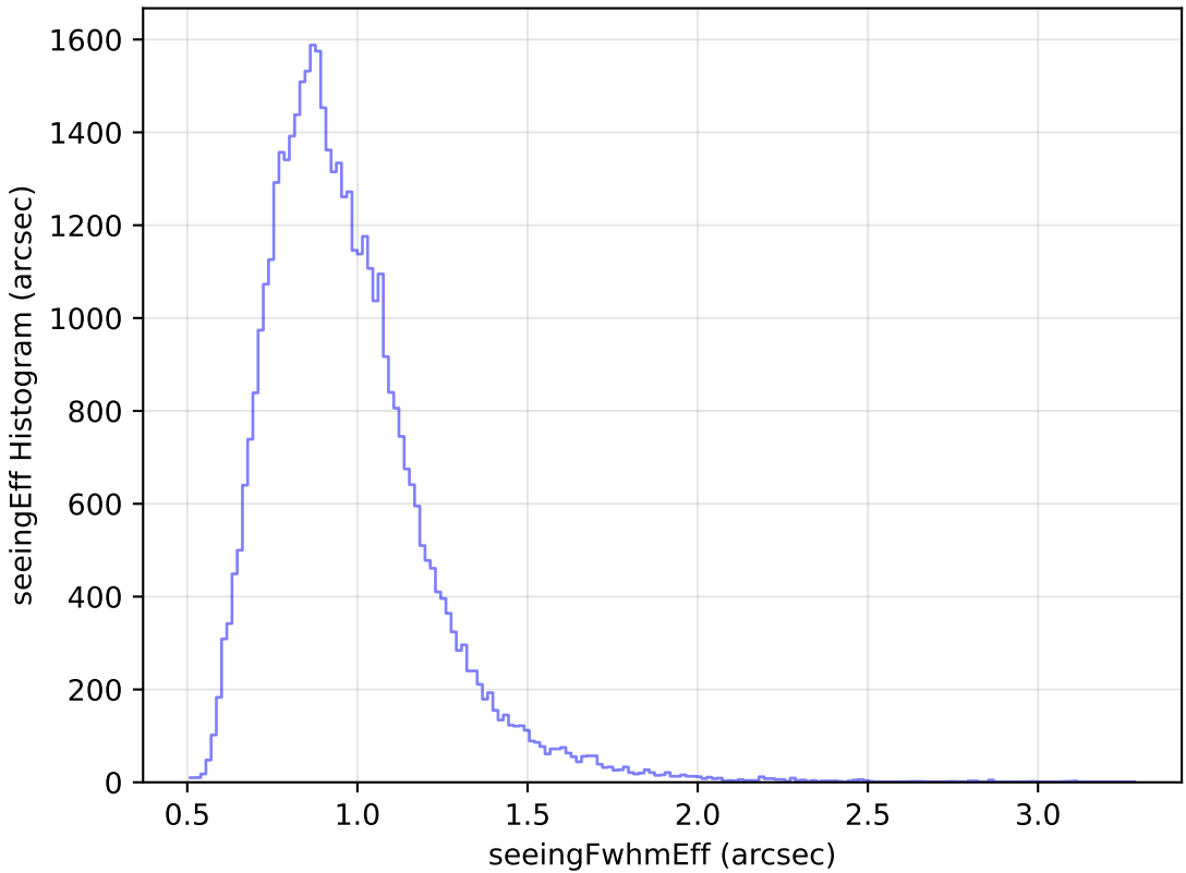
noroll_mjdp365_v3.4_10yrs Yr 1 y band: seeingEff Histogram
