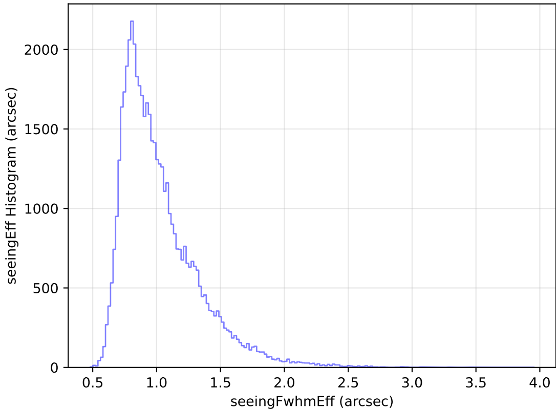
noroll_mjdp365_v3.4_10yrs Yr 1 r band: seeingEff Histogram
