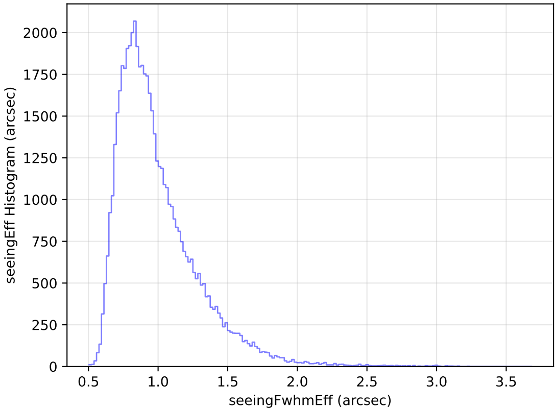
noroll_mjdp365_v3.4_10yrs Yr 1 i band: seeingEff Histogram
