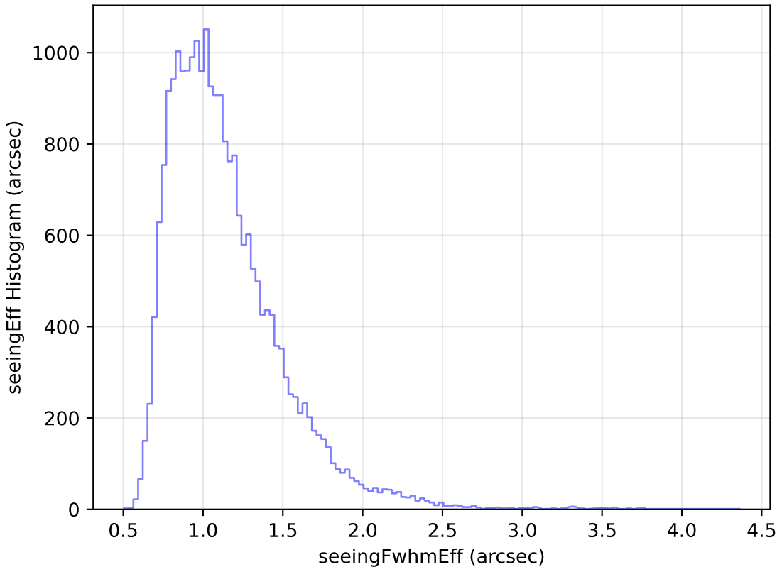
noroll_mjdp365_v3.4_10yrs Yr 1 g band: seeingEff Histogram
